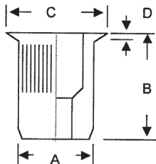
COUNTERSINK
